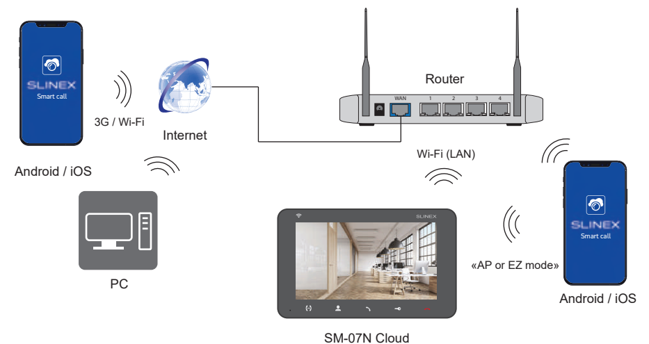
Diagram 2. SM-07N Cloud wireless Wi-Fi network connection.
