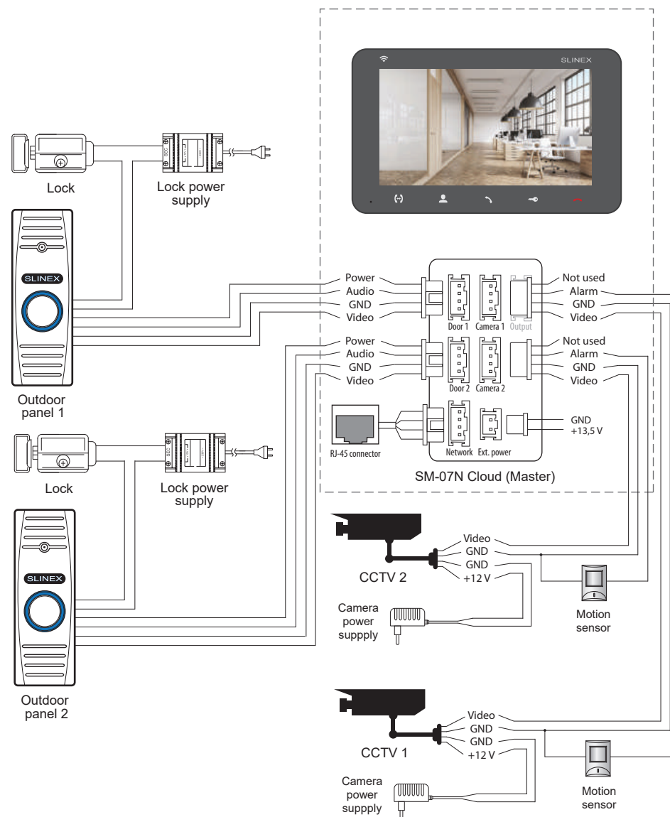
Diagram 1. Outdoor panels, cameras and locks connection.
