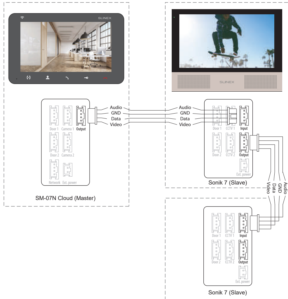
Diagram 2. SM-07N Cloud and Sonik 7 monitors connection into one system.
